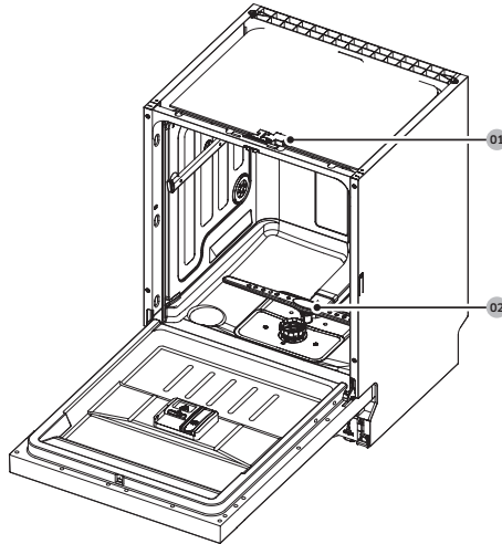
02 Lower nozzle
