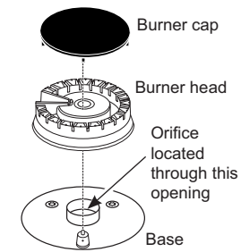
Round burner
